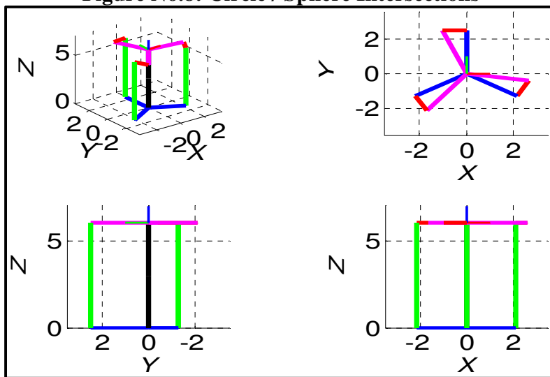
Figure No.9a: Nominal Orientation Example 1: Solution a Elbow Up
