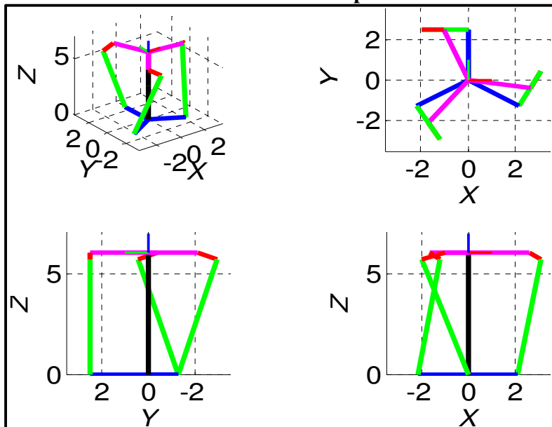
Figure No.9b: Nominal Orientation Example 1: Solution b Elbow Down
