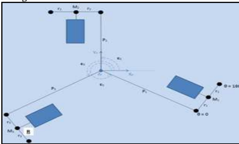
Figure No.6: Moving Platform Kinematic Details
