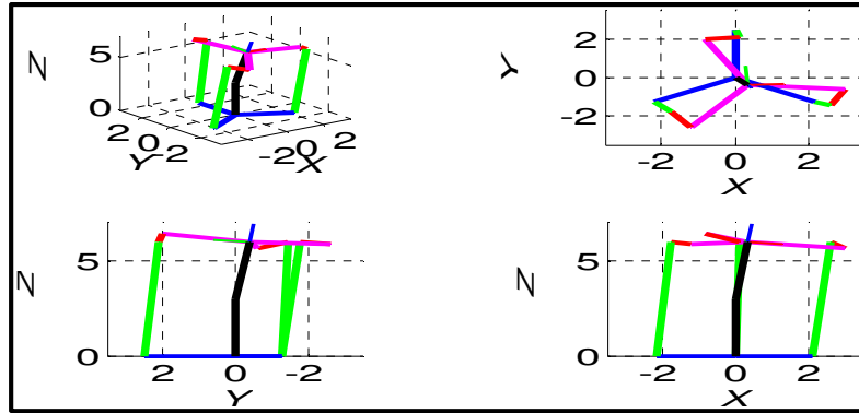
Figure No.10a: Nominal Orientation Example 2: Solution a Elbow Up
