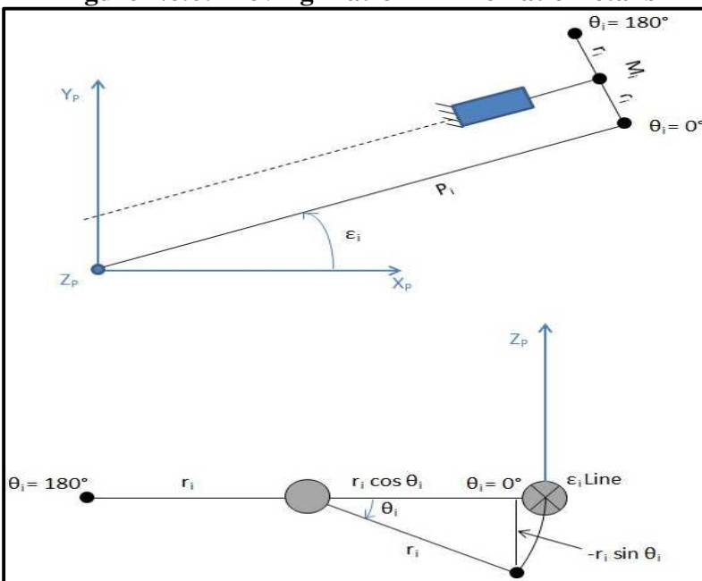
Figure No.7: \{^P r_i\} Kinematic Details
