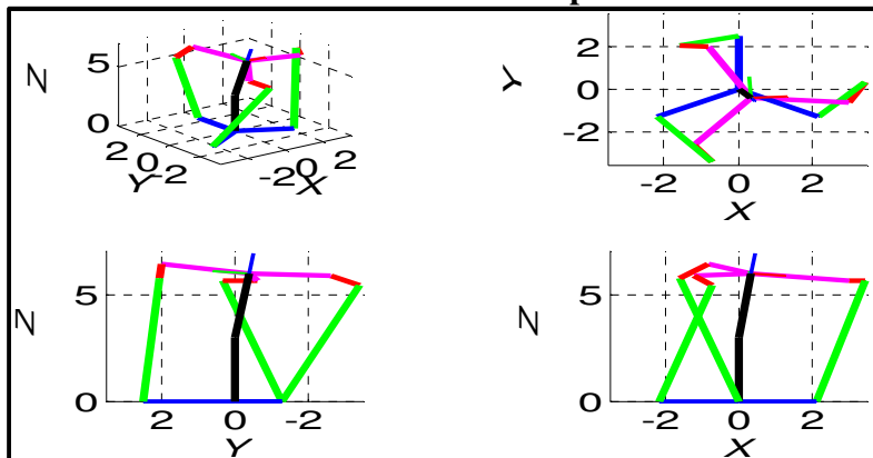
Figure No.10b: Nominal Orientation Example 2: Solution b Elbow Down
