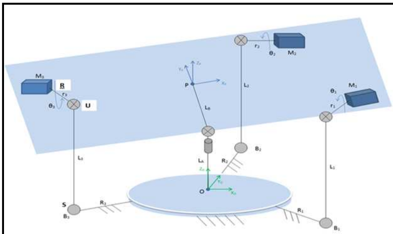
Figure No.4: Three-dof 3-SUR1-RU Parallel Platform Robot Kinematic Diagram
